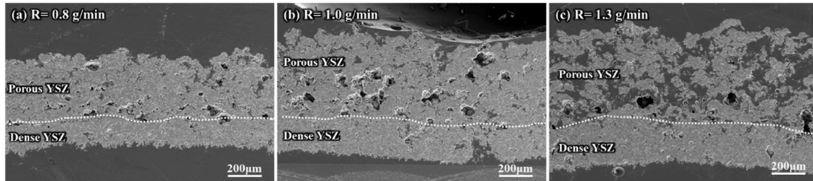
Fig. 9. Cross-sectional images of double-layered TBC depending on the PEEK feed rate R (a) 0.8 g/min, (b) 1.0 g/min, and (c) 1.3 g/min (PEEK feed distance D = 5 cm).
