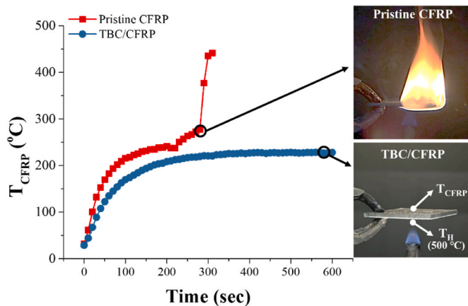
Fig. 13. The back-face surface temperature of the CFRP and TBC/CFRP composites during the thermal shock test.
