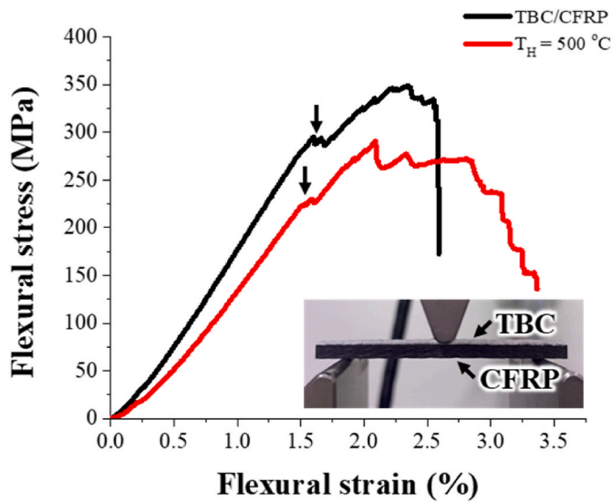
Fig. 15. Flexural stress-strain curve of TBC/CFRP composites before and after thermal shock test ( T_H = 500^\circ\text{C} ).
