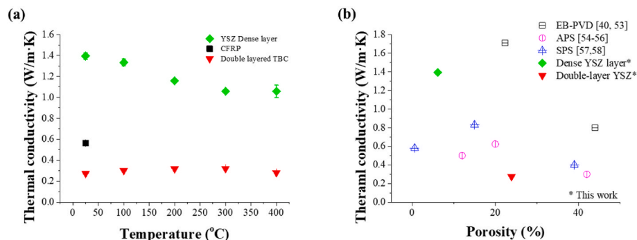
Fig. 12. Comparison of thermal conductivity between (a) TBC/CFRP composite and (b) porous YSZ coating from other references. Double layered TBC made with D = 5 cm and R = 1.0 g/min.
