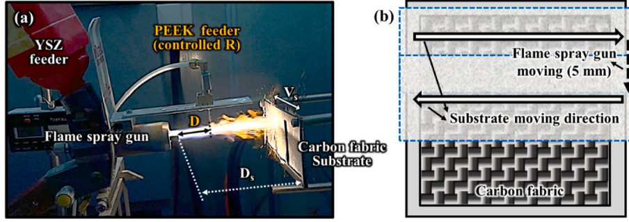
Fig. 1. (a) Experimental setup of flame spraying and (b) coating pattern.
