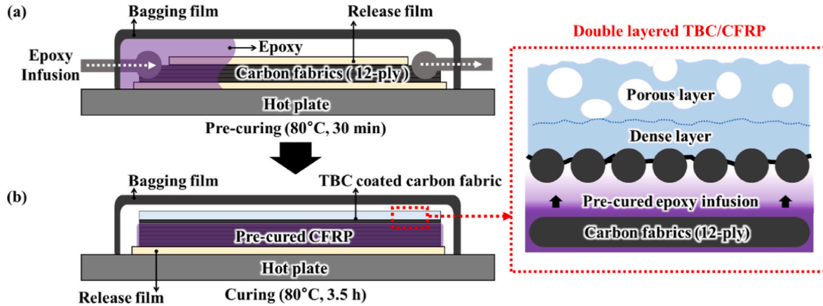
Fig. 3. Schematic of TBC/CFRP composite manufacturing process: (a) precuring process of the CFRP substrate and (b) post-curing of the TBC/CFRP composite.
