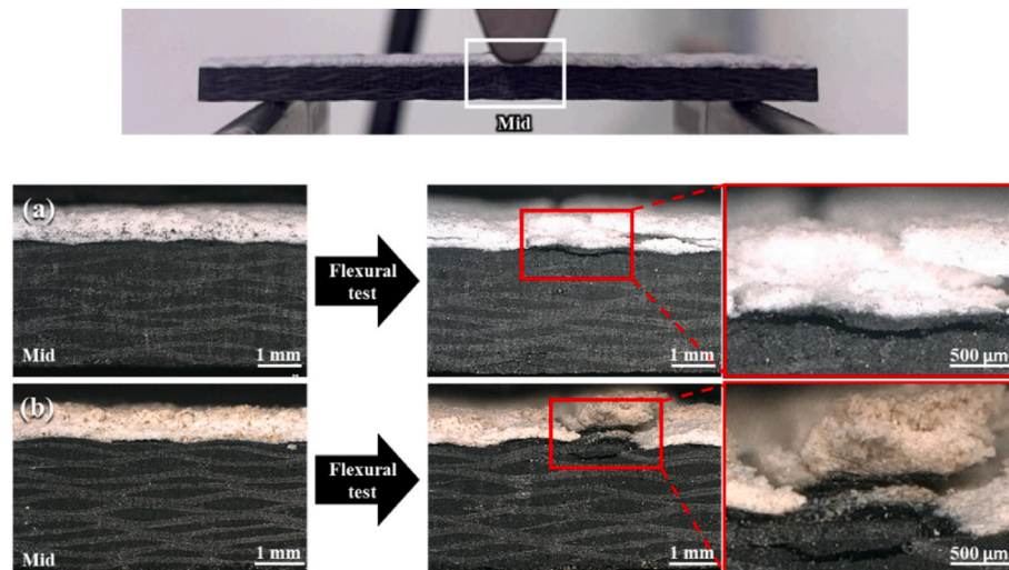
Fig. 17. Cross-sectional images of TBC/CFRP specimens before and after three-point bending test: (a) before and (b) after thermal shock test.
