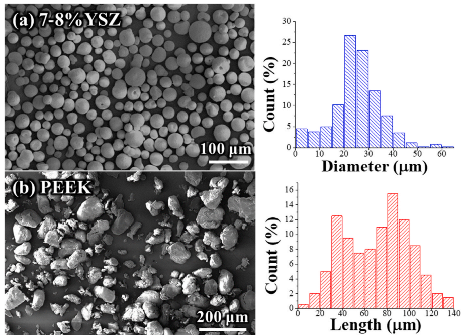
Fig. 5. SEM images and particle size distribution of (a) YSZ (used as a thermal barrier material) and (b) PEEK (used as a pore-forming agent).
