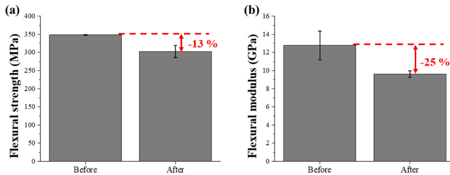
Fig. 16. Comparison of (a) flexural strength and (b) flexural modulus of TBC/CFRP specimen after thermal shock ( T_H = 500^\circ\text{C} ).
