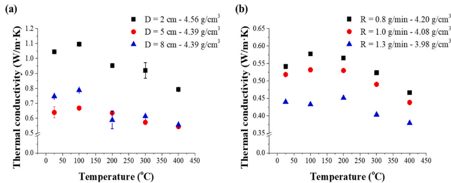
Fig. 11. Effects of PEEK feed distance D and rate R on the thermal conductivity of porous YSZ layers prepared with (a) D = 2–8 cm with R = 0.3 g/min and (b) R = 0.8–1.3 g/min with D = 5 cm.
