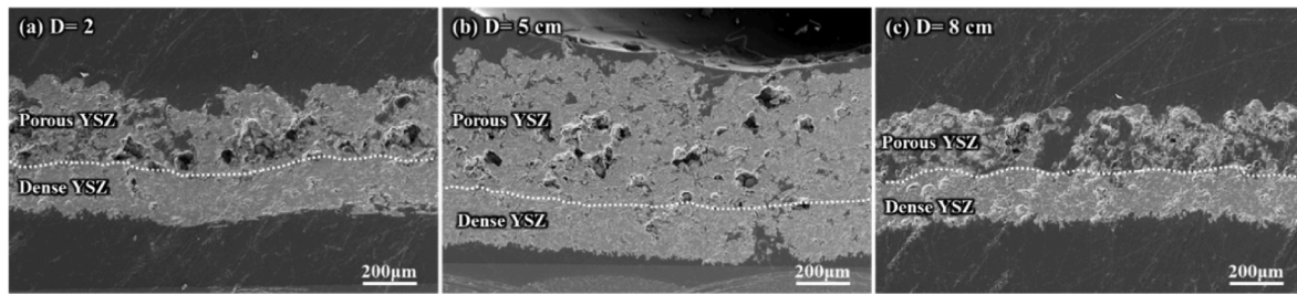
Fig. 8. Cross-sectional observation of a double-layered TBC layer fabricated at various PEEK injection distances D : (a) 2 cm, (b) 5 cm, and (c) 8 cm (PEEK feed rate R = 1.0 g/min).
