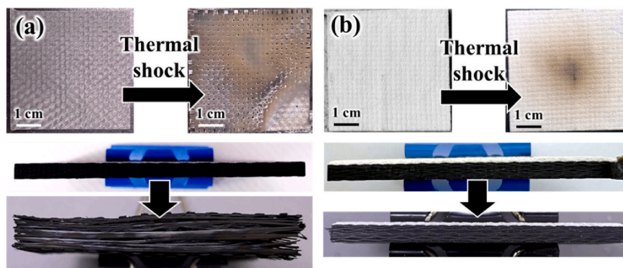
Fig. 14. Macroscopic images of thermal shock-tested (a) pristine CFRP and (b) TBC/CFRP composites.
