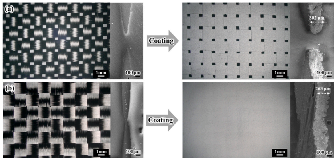
Fig. 6. Effect of desizing on TBC surface morphology: (a) pristine and (b) desized CF substrates. Only YSZ particles were flame sprayed for four passes with D_s = 14 cm.
