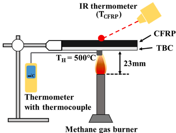
Fig. 4. Schematic of the thermal shock test.
