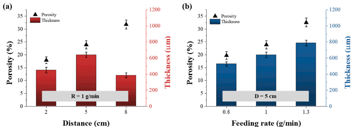
Fig. 10. Porosity and thickness of the double-layered TBC as a function of (a) D and (b) R .
