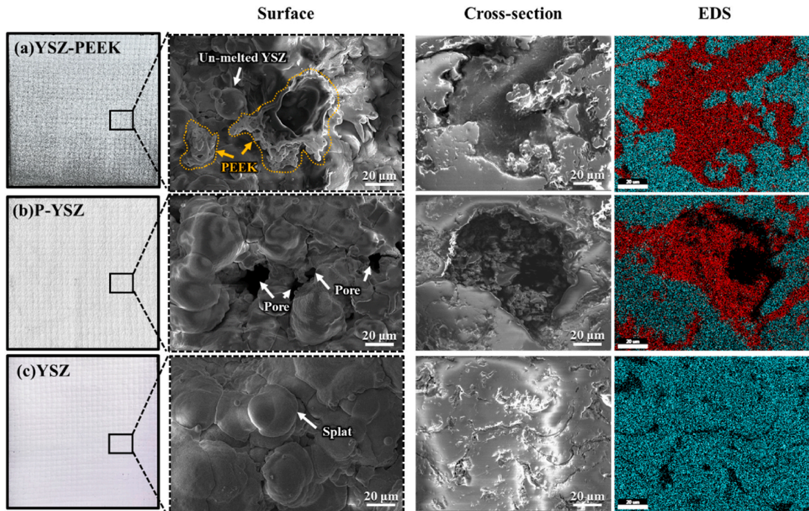
Fig. 7. Visual inspection, SEM images and energy-dispersive X-ray element mapping of C (PEEK-red) and Zr (blue) in (a) YSZ-PEEK layer, (b) heat-treated co-sprayed YSZ-PEEK layers ( D = 5 cm and R = 1.0 g/min) and (c) sprayed YSZ layer ( D_s = 14 cm). For interpretation of the references to color in this figure legend, the reader is referred to the Web version of this article.
