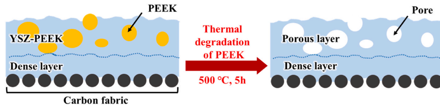
Fig. 2. Schematic of double-layered TBC fabrication.
