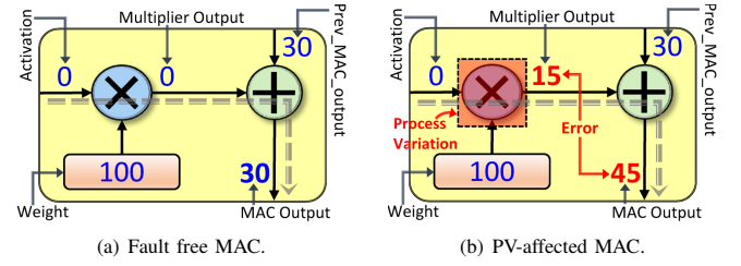
Fig. 6: Working of a PV-free and PV-affected MAC.
