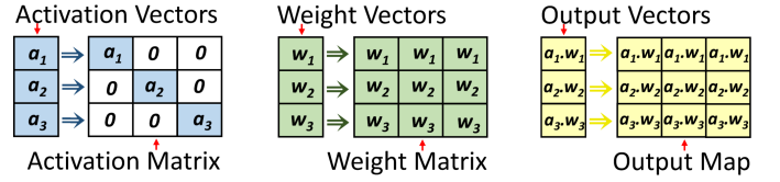
Fig. 7: Development of input matrices and output map—correct outputs—by FCU.
